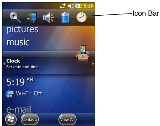
Figure 2-8 Icon Bar
