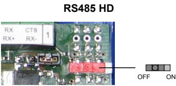
Figure 9 – RS485 HD Termination Resistance Switch
