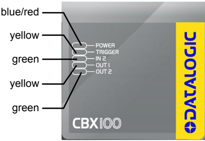
Figure 11 – Indicator LEDs
