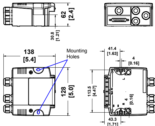
Figure 1 - Overall Dimensions
