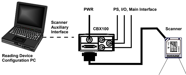
Figure 2 – System Layout
