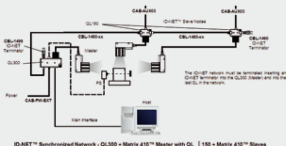
ID-NET™ Synchronized Network - QL300 + Matrix 410™ Master with QL | 150 + Matrix 410™ Slaves
